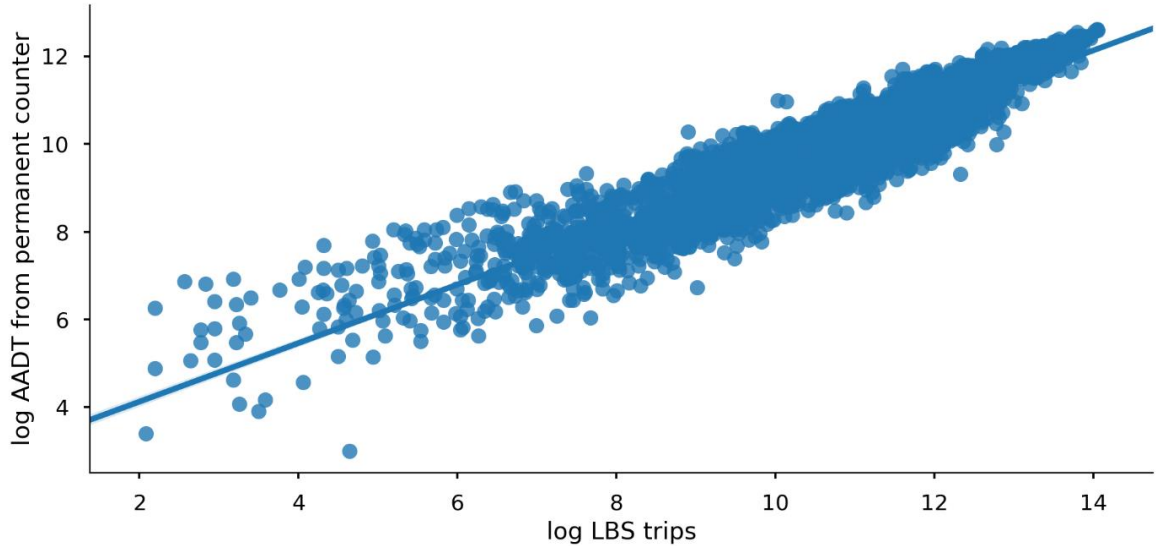
Figure 4: Correlation of population-normalized LBS to permanent loop counter data – the single best predictor value. The rest of the machine-learning work aimed at improving over these results.
